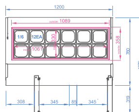
SHR12-2
