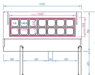
SHR15-2
