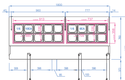
SHR18-3
