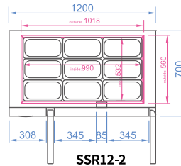
SSR12-2
